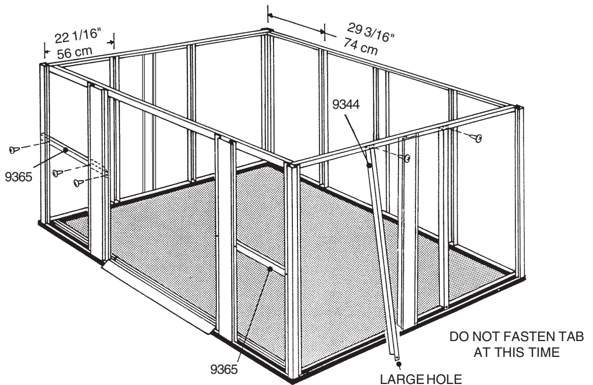
FASTEN STUD AT LOWER HOLE
