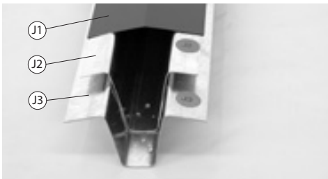
Firstabdeckung (J1) roof ridge cover (J1) Firstträger oben (J2) upper roof ridge beam (J2) Firstträger unten (J3) lower roof ridge beam (J3) couverture de faitière (J1) copertura colmo (J1) poutre de faitage sup. (J2) supporto colmo superiore (J2) poutre de faitage inf. (J3) supporto colmo inferiore (J3)
